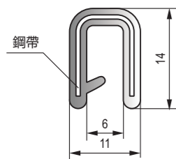
D-028 PVC裝飾條 PVC trim strip
