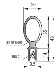
DFT-023 黑色EPDM鋼片密封條 Black EPDM sealing strip(with steel sheet)
