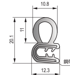
DFT-011 黑色EPDM鋼帶密封條 Black EPDM sealing strip(with steel sheet)
