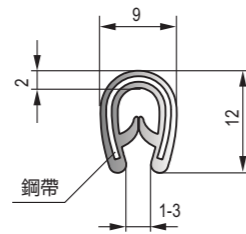
D-026 PVC裝飾條 PVC trim strip
