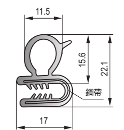
DFT-012 黑色EPDM鋼帶密封條 Black EPDM sealing strip(with steel sheet)
