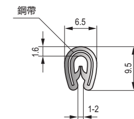
D-024 PVC裝飾條 PVC trim strip
