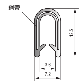
D-021 PVC裝飾條 PVC trim strip
