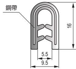
D-025 PVC裝飾條 PVC trim strip
