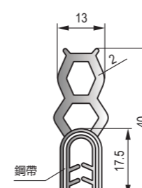
DFT-022 黑色EPDM鋼帶密封條 Black EPDM sealing strip(with steel sheet)
