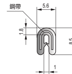
D-023 PVC裝飾條 PVC trim strip
