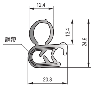
DFT-013 黑色EPDM鋼帶密封條 Black EPDM sealing strip(with steel sheet)
