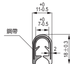
D-029 PVC裝飾條 PVC trim strip
