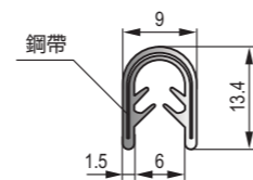
D-030 PVC裝飾條 PVC trim strip
