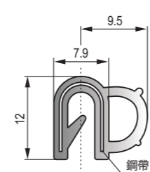
DFT-018 黑色EPDM鋼帶密封條 Black EPDM sealing strip(with steel sheet)
