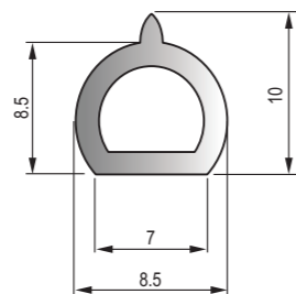
DFT-065 PVC密封膠條 PVC gasketing
